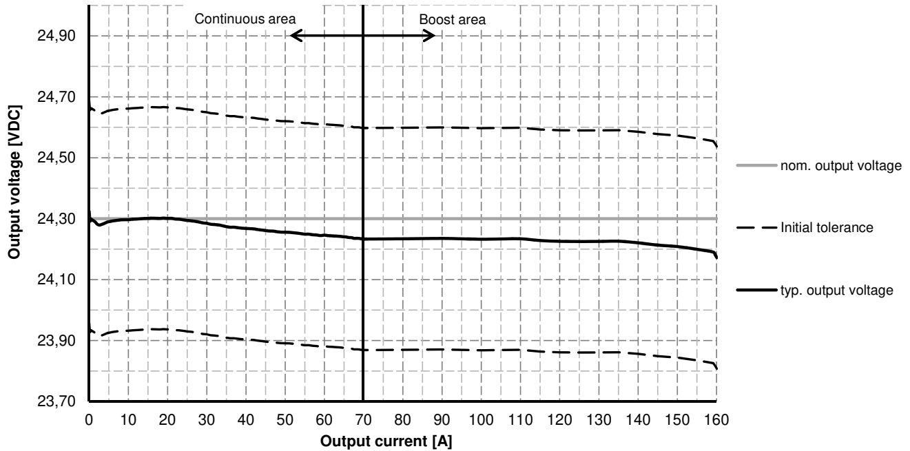
Figure 8.7: Typ. output voltage and initial tolerance
